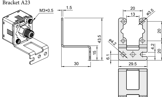
Bracket A23
