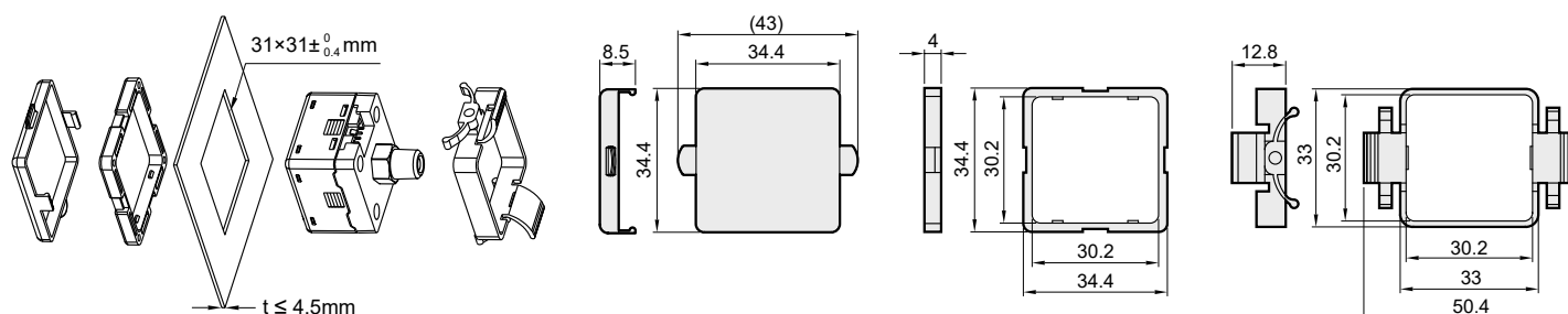
Panel mounting adapter with protective cover C2
