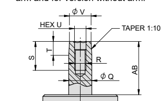
Piston rod end detail for double-sided arm:
