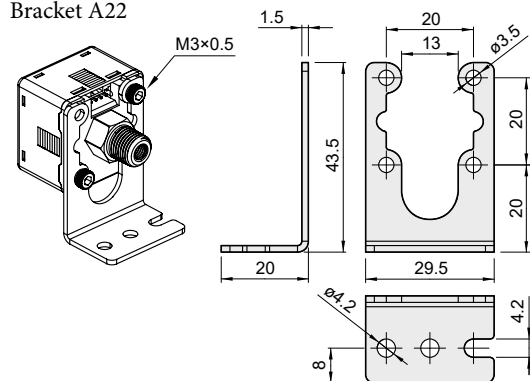
Bracket A22
