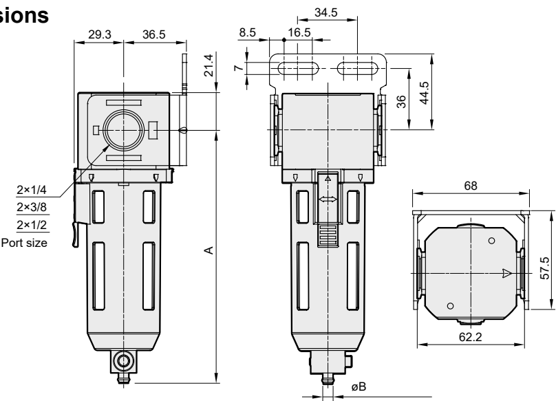
Semiautomatic condensation draining
